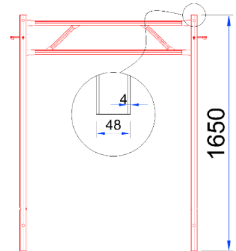
Telescopic Frame
